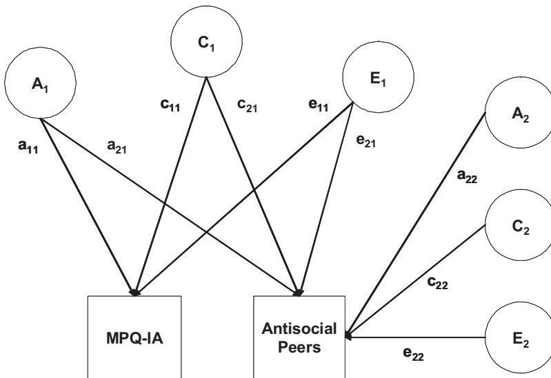
Figure 1. Path diagram of a bivariate ACE Cholesky model for MPQ Impulsive Antisociality (MPQ-IA) and antisocial peers (AP). This model decomposes the variance into additive genetic ( A_1 , A_2 ), shared environmental ( C_1 , C_2 ), and nonshared environmental ( E_1 , E_2 ) effects. a_{11} , c_{11} , and e_{11} are paths representing effects on MPQ-IA only. a_{21} , c_{21} , and e_{21} are effects on MPQ-IA that also contribute to AP. a_{22} , c_{22} , and e_{22} are effects that are unique to AP.
